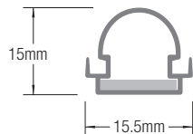
Extrusion profile
